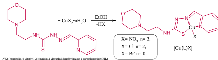
Figure 3. Synthesis scheme of Cu(II) coordination compounds with HL
