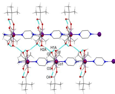
Figure 1. Structure of the 1D chains in 1 .
