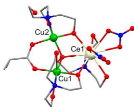
Figure 2. Structure of the cationic complex [CeCu 2 (ib)(NO 3 ) 2 (H 2 tea) 3 ] +
